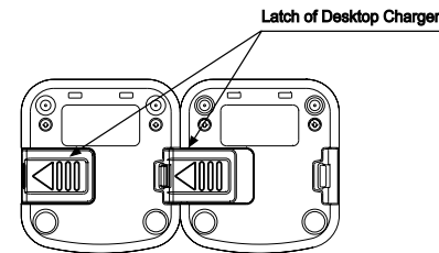
Figure 2 Diagram of Multi-Unit Charger Assembly
